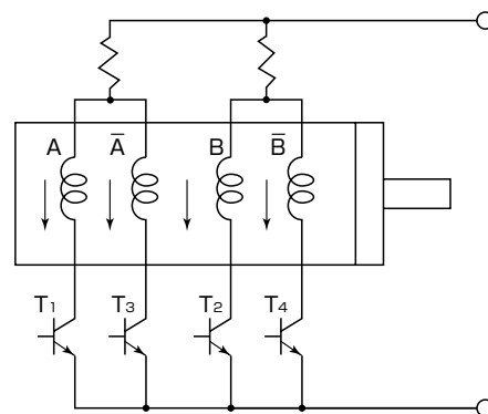
Figure 1 Unipolar Drive
