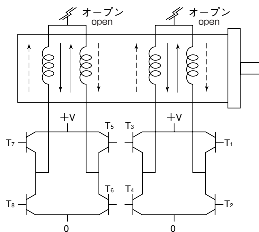
Figure 2 Bipolar Drive
